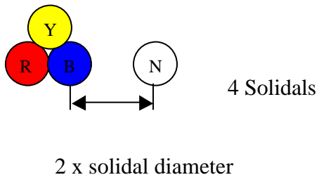
FIGURE A1 Trefoil Configuration – laid direct in ground or in air
