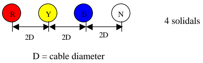
FIGURE A2 Flat Configuration – laid direct in ground or in air
