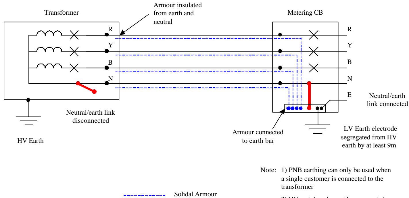
FIGURE B3 Solidal Bonding Requirements – Arrangement 3 with segregated HV/LV earthing and a PNB connection
