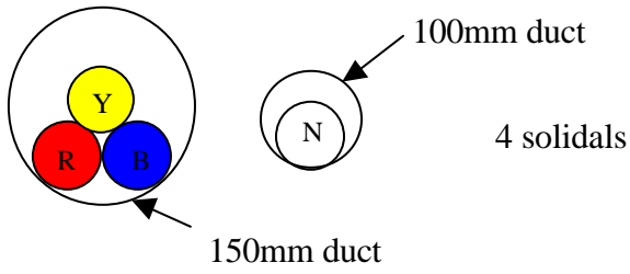
FIGURE A3 Trefiol Configuration – laid in ducts
