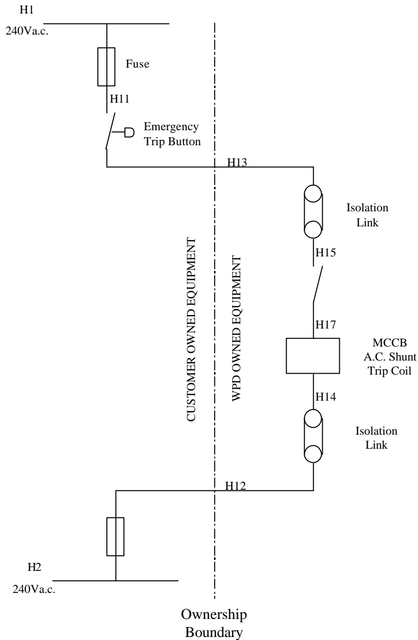
FIGURE 5 Remote Emergency Tripping
