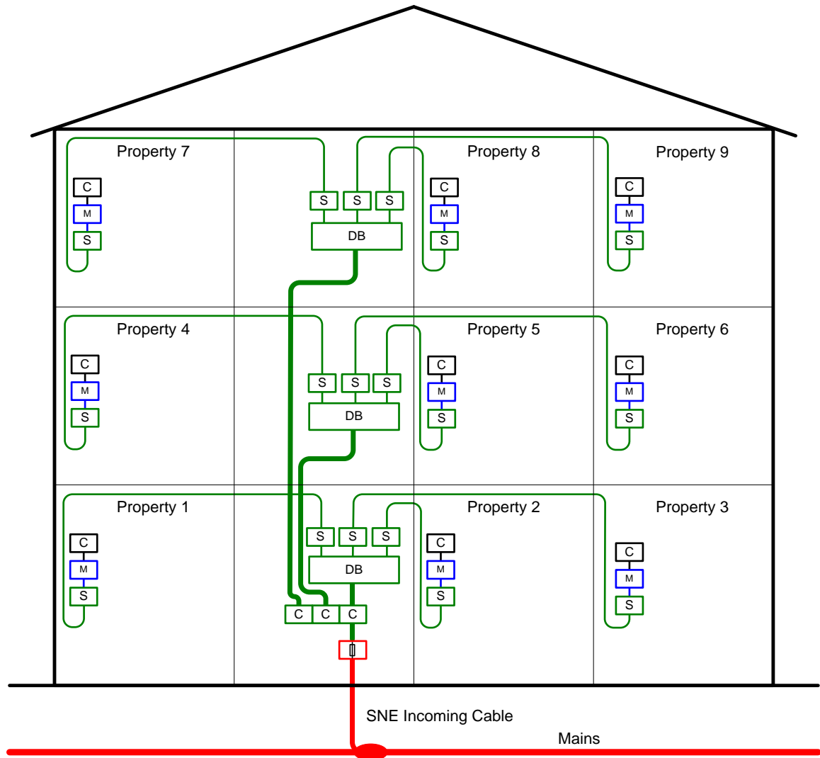
Figure 3B Option 3B; Services Originating from within a Building Network – Single Incoming Circuit - Metering at Individual Properties
