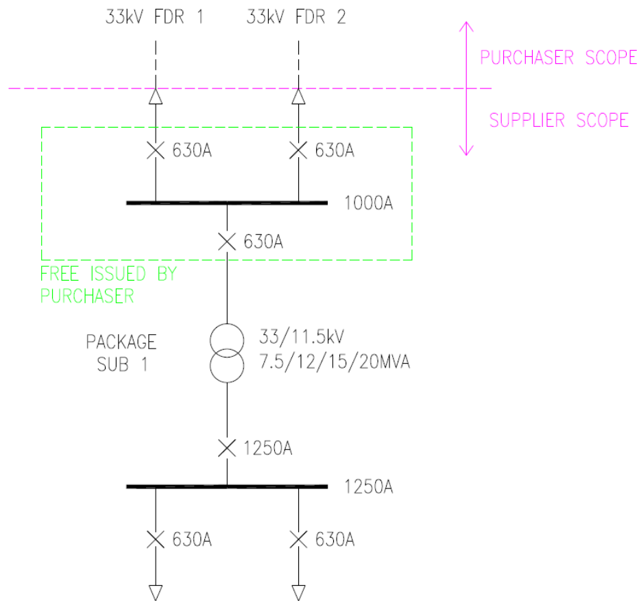
Figure 3.1 Indicative demarcation between Purchaser and Supplier SoW
