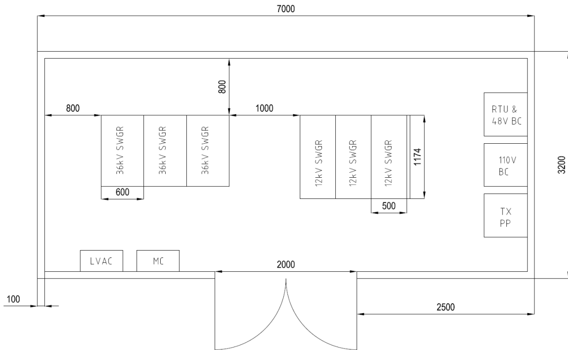
Figure 8.1 Indicative enclosure layout
