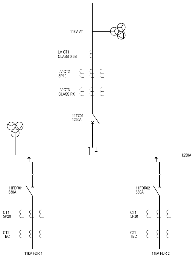
Figure 7.1 12kV switchgear configuration
