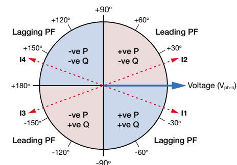
Figure 1: Four Quadrant Diagram - Direction of Power Flow
