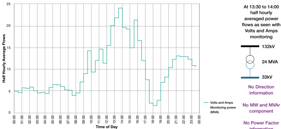
Figure 3: Power flow represented with Amps and volts metering
