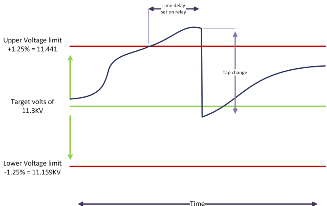
Figure A10 Operation of Tap-change Control Relay
