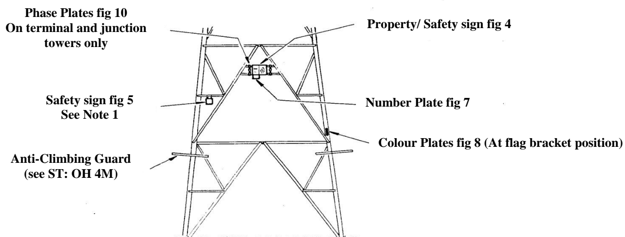
Position of Circuit Identification Colour Plates
